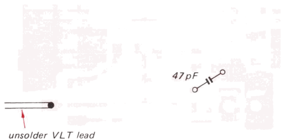
Fig. 3-10 Dummy antenna 47 pF on sw front end
