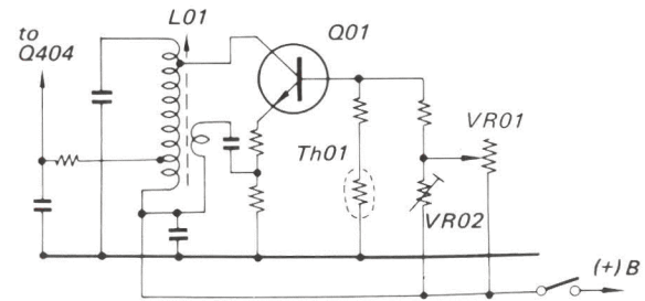
Fig. 1-7 BFO circuit
