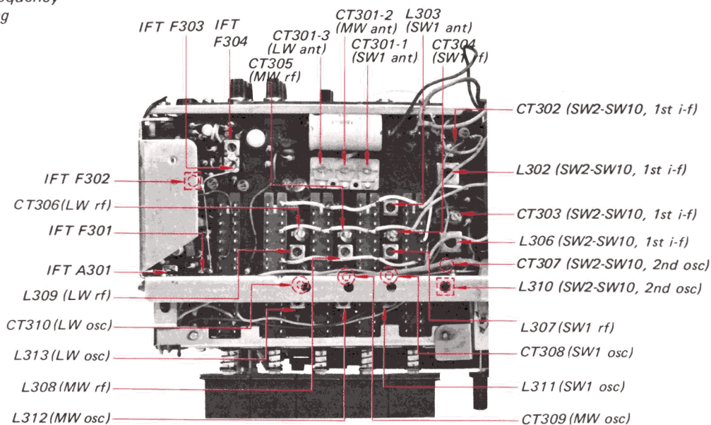
Fig. 3-12 Cp/i-f circuit board adjustments
