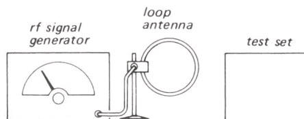
Fig. 3-17 BFO adjustment setup
