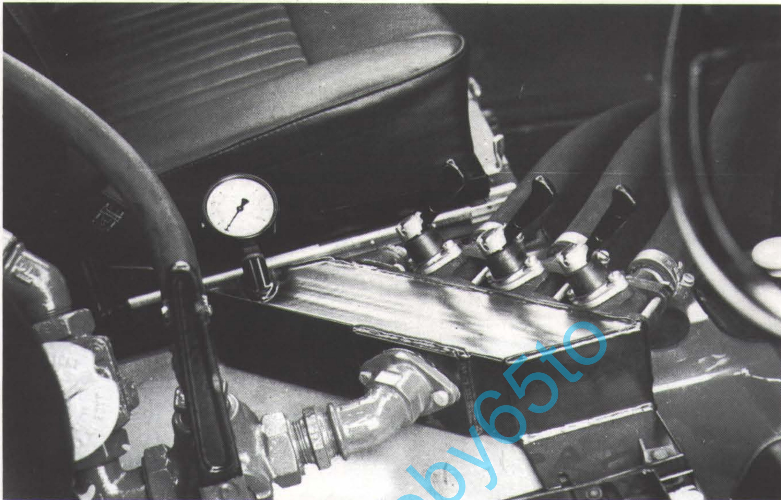
Cab-control unit showing ease of access to pressure control valve and cocks and clear pressure gauge visibility
